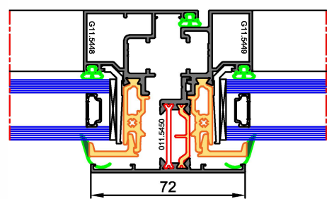
Battent CENTRAL PF serrure
