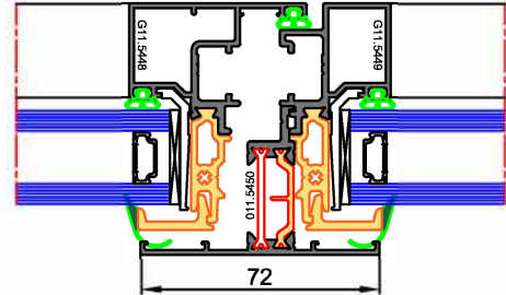
Battement CENTRAL OF
